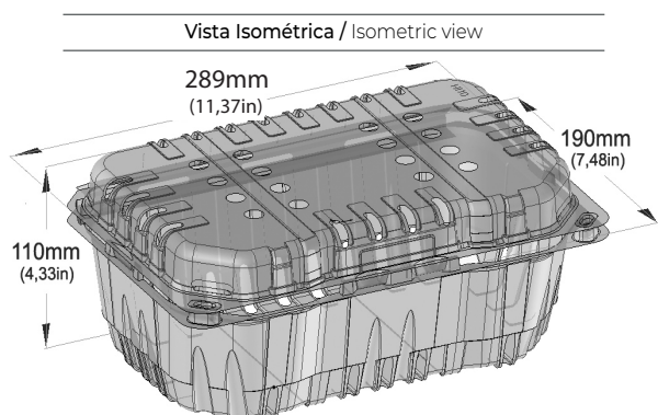
Vista Clamshell abierto / View of open Clamshell
